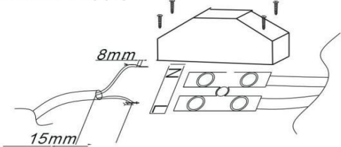
Electrical Supply
