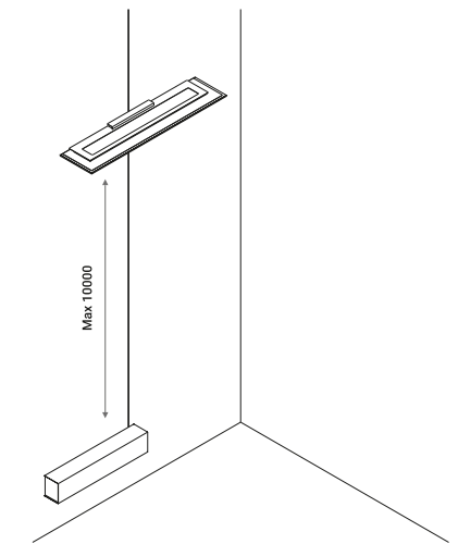
REFLEX: example of installation with wall/ceiling driver
