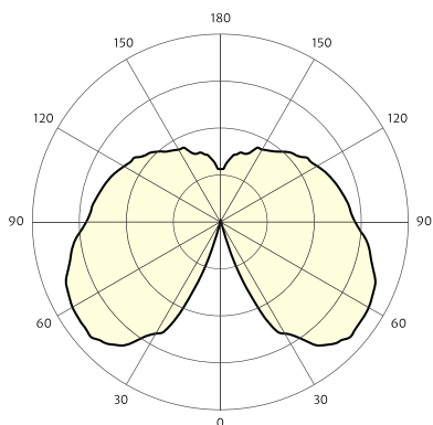
Smoked bulb - Light Intensity distribution
