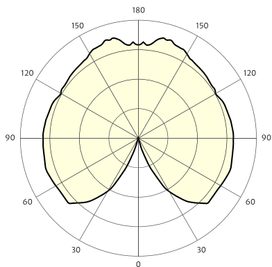
Clear bulb - Light Intensity distribution
