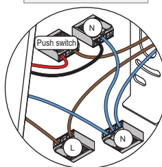
2.b PUSHDIM DIAGRAM
