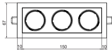
bottom view
