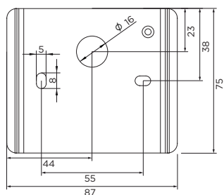
mounting base dimensions
