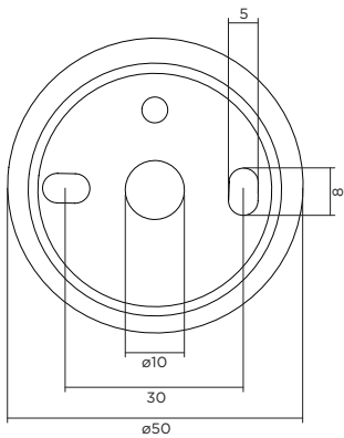
base plate dimensions
