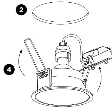
Wired springs
