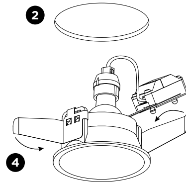
Blade springs
