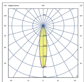
Aluminium optic 20°
