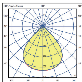
Nylon optic 85°
