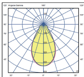
Methacrylate optic 60°
