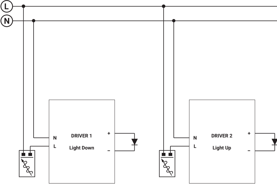
Example connection (optional) for dimming TRIAC/IGBT
