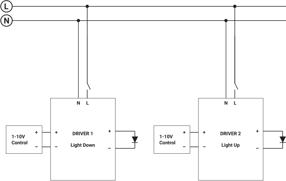
Example connection (optional) for dimming 1-10V
