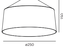
SHADE 2.0
