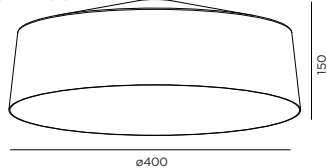
SHADE 3.0
