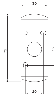
Mounting base:
