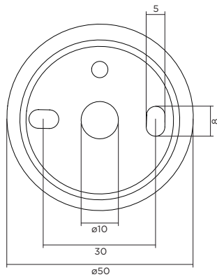
ceiling base dimensions
