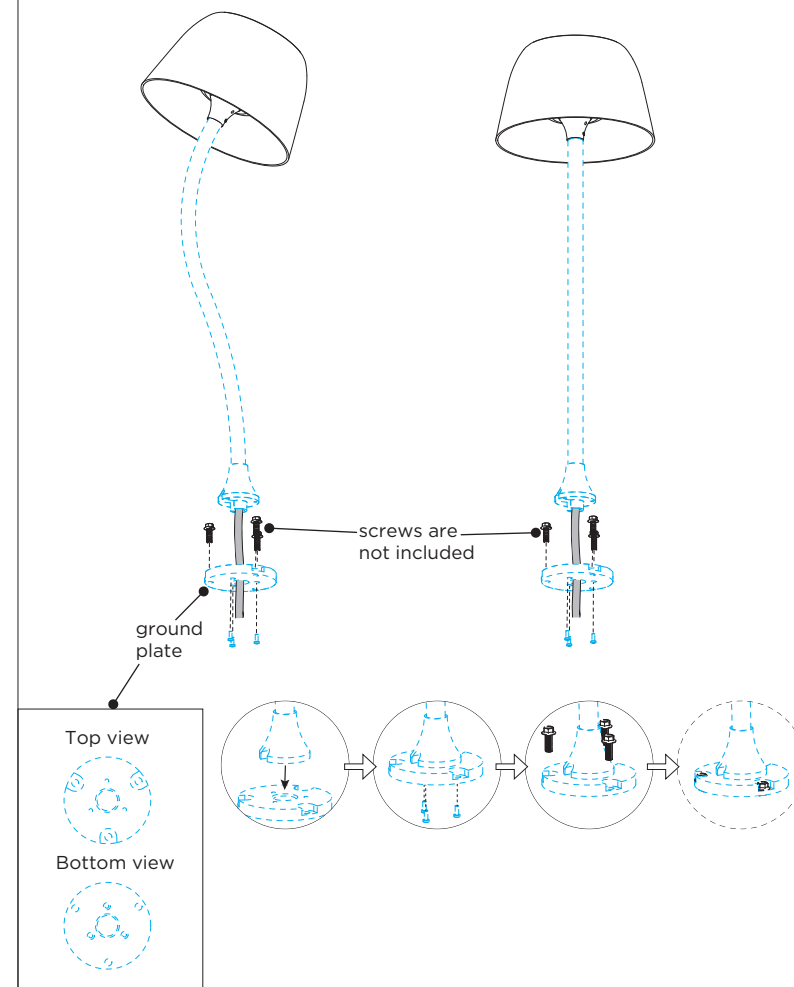
installation with ground plate
