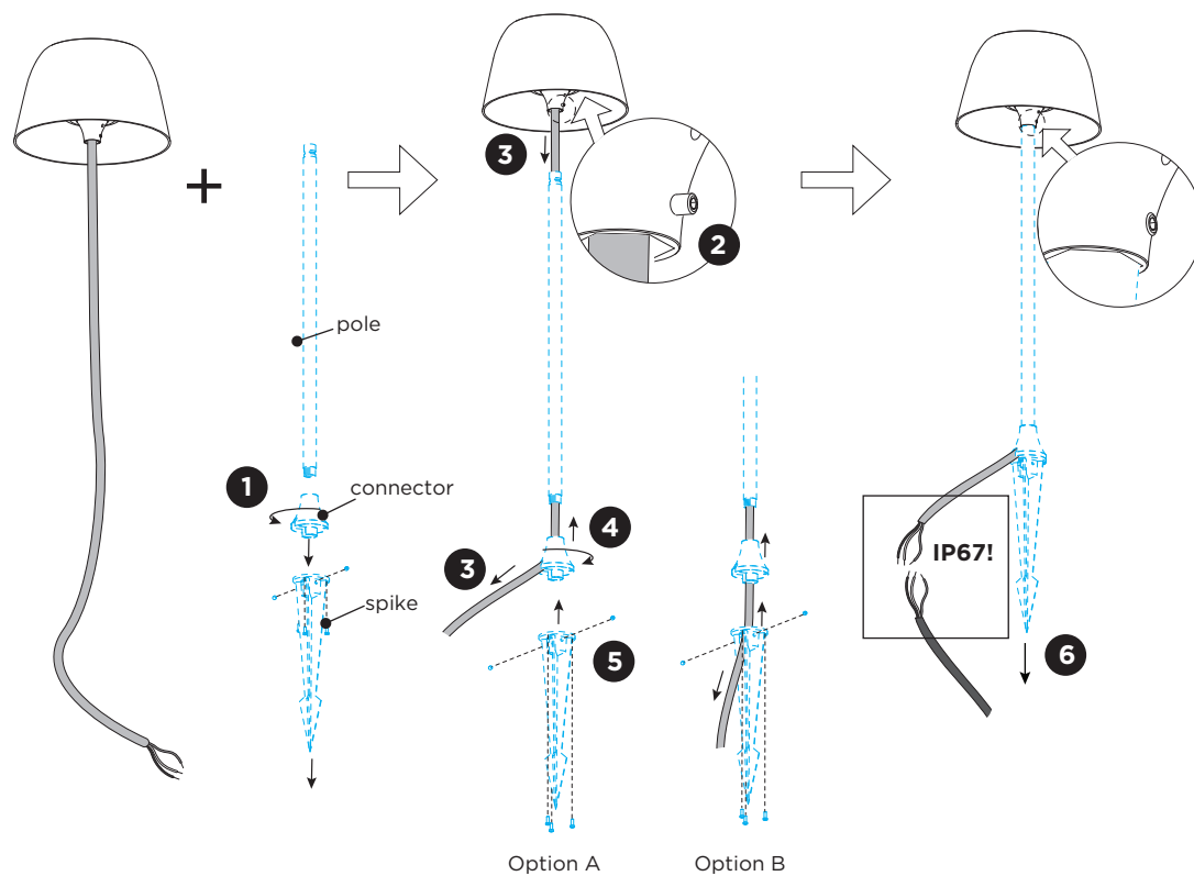
installation with straight post
