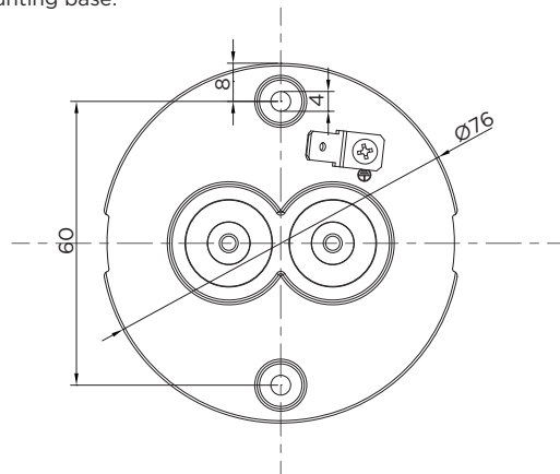
Mounting base:
