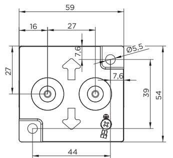
Mounting base:
