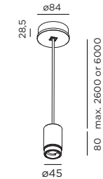
WIRO SUSPENSION SINGLE without steel wire
